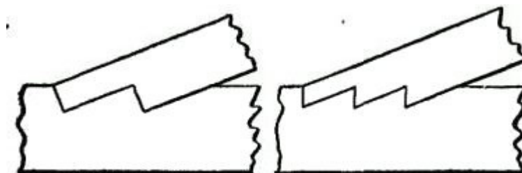
Fig. 297. Heel Joints.
