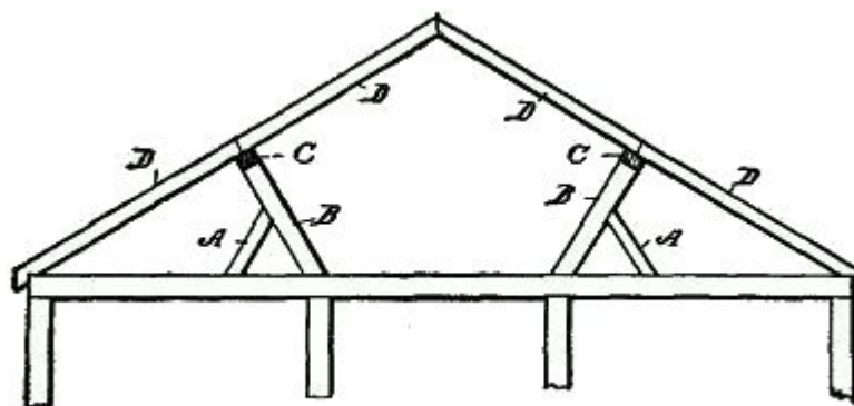
Fig. 285. Purlin Roof.
