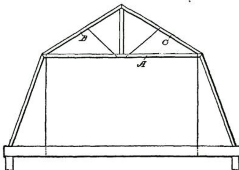
Fig. 288. The Mansard.
