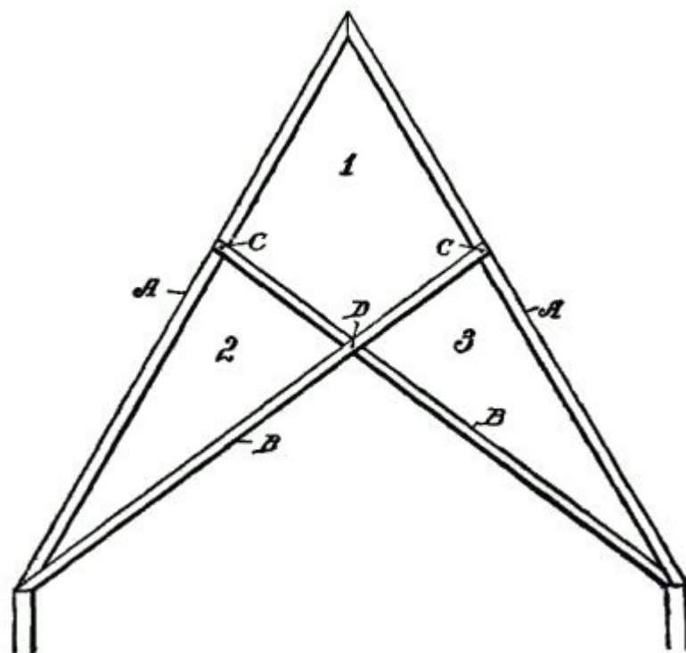
Fig. 289. Scissors Beam.
