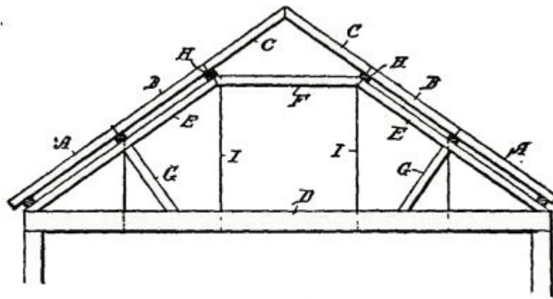
Fig. 286. Princess Truss.
