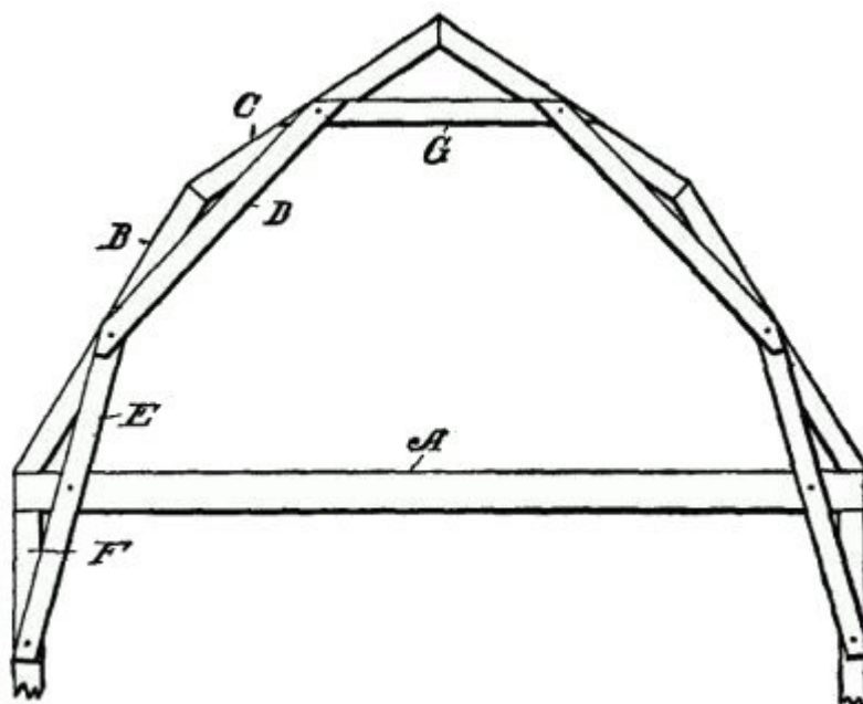
Fig. 284. Gambrel Roof.
