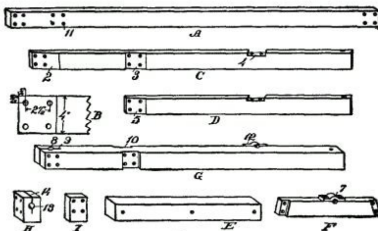
Fig. 241. Frame details.
