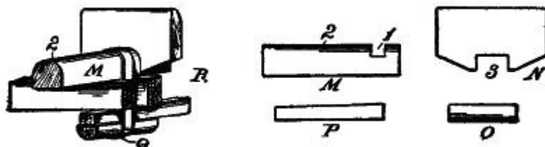
Fig 243. Tool Rest.
